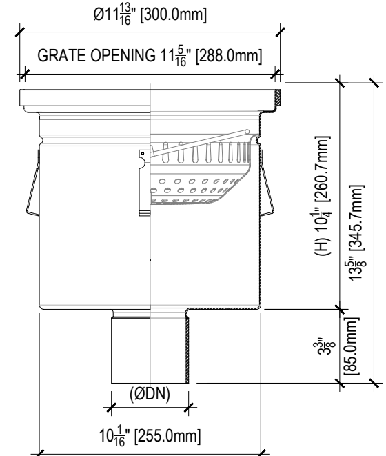
DV1-12-9: PARTIAL SECTION
